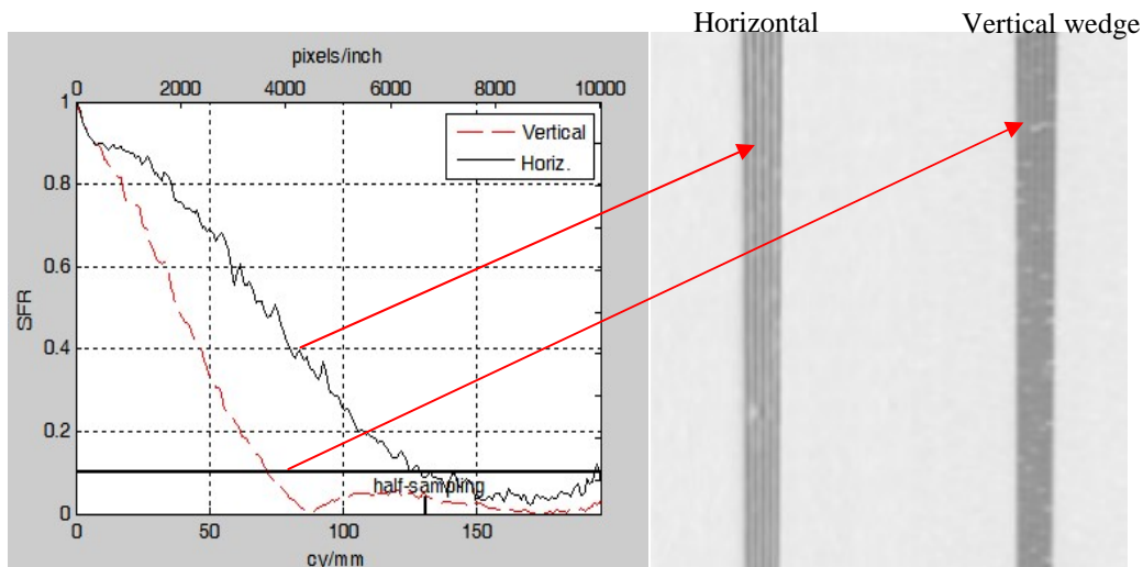
Fig. 4.11 – SFR differences due to scanning motion
