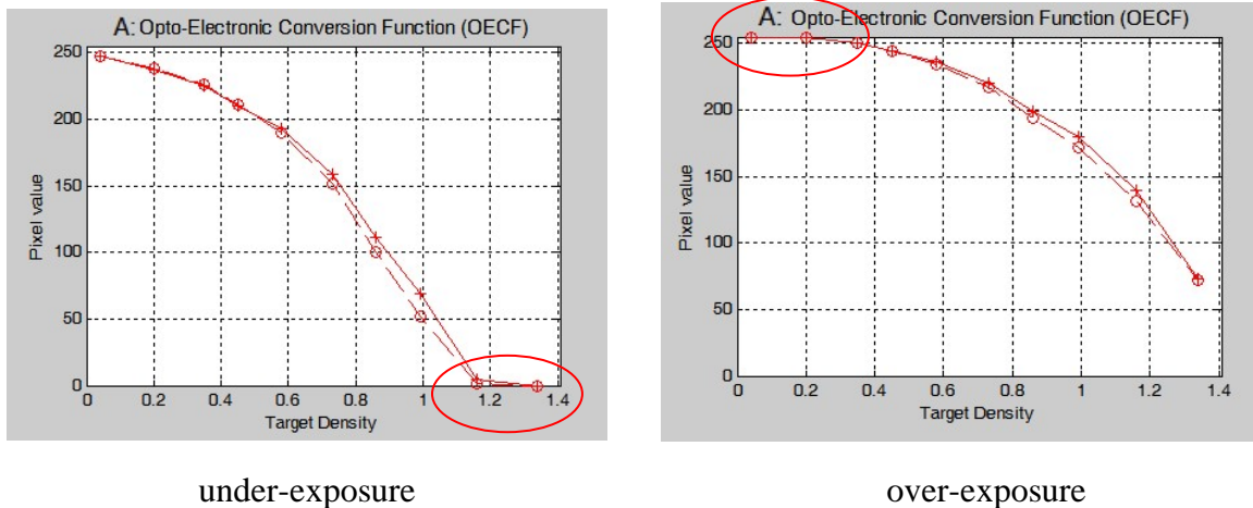
Fig. 4.2 – Examples of acceptable OECF curves that satisfy the discrimination and monotonic criteria. Note lack of pixel value buffer at high density region
