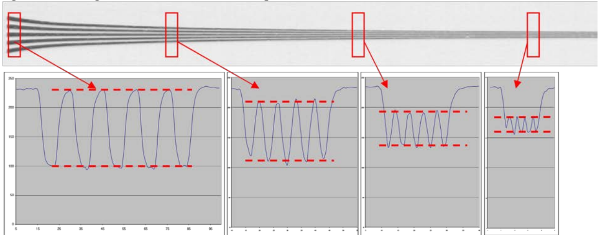
Fig. 4.8 – Indication of how feature contrast is reduced as spatial frequency increases.
