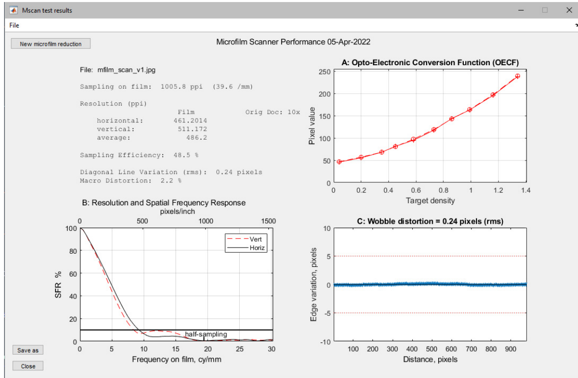
Fig. 4.1 - Typical performance results panel from Mscan software
