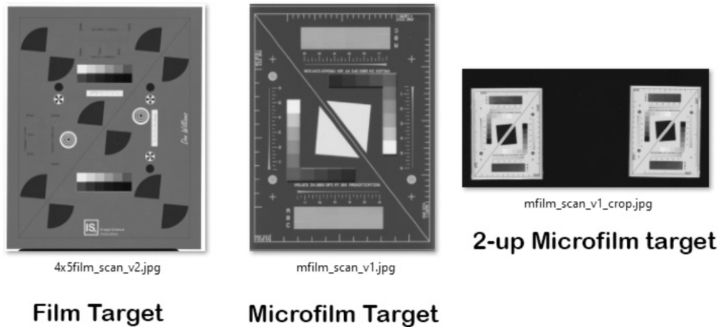
Figure 1: The target types, (L-R) 4x5 film target, Microfilm target, and 2-up version of the microfilm target.
