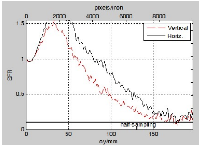
Fig. 4.10 – Illustration of sharpening signatures manifested in the SFR response (left). Note the greater than 1.00 SFR response. Such aggressive sharpening often leads to haloes at light to dark transitions as illustrated in the example on the right.
