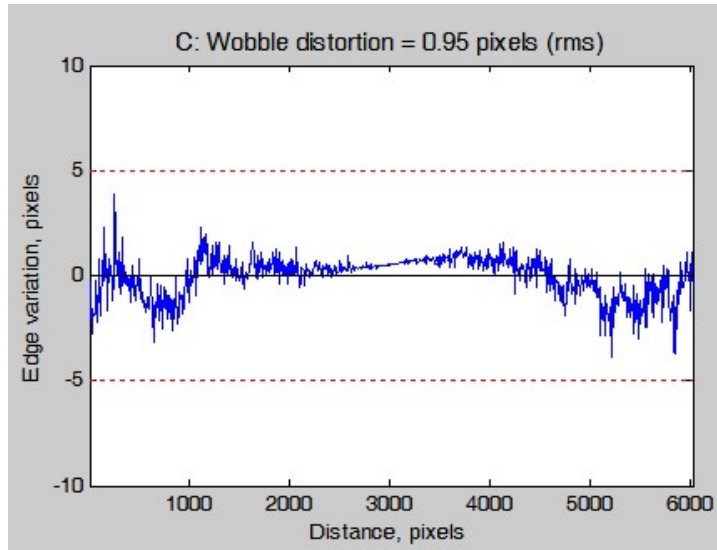
Fig. 4.13 – Micro or wobble distortion graph
