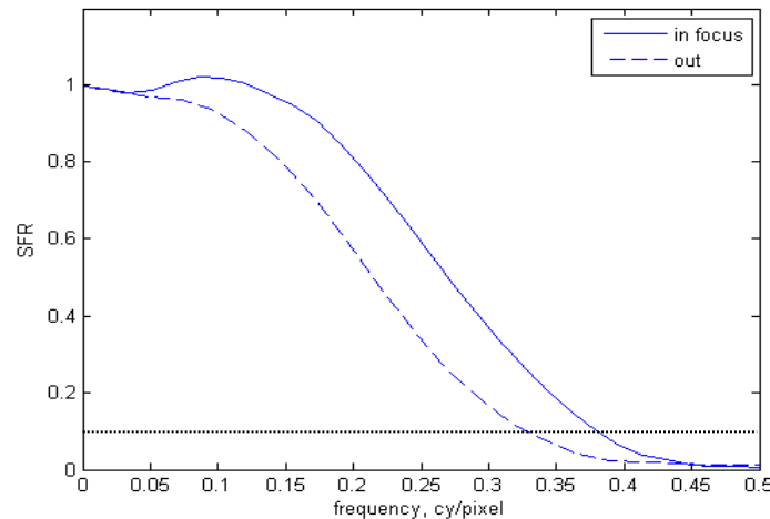
Figure 1. SFR measurement results for a digital camera with two lens focus positions.
