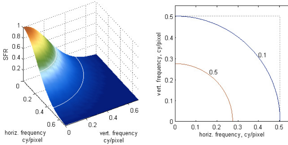
Figure 4. Example of two-dimensional symmetric SFR and corresponding 50% and 10% response contours.
