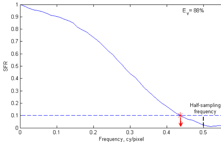
Figure 3. Results of 10% SFR calculation as in Fig. 2.
