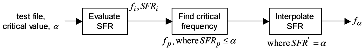
Figure 2. Calculation of limiting resolution (frequency) from SFR.
